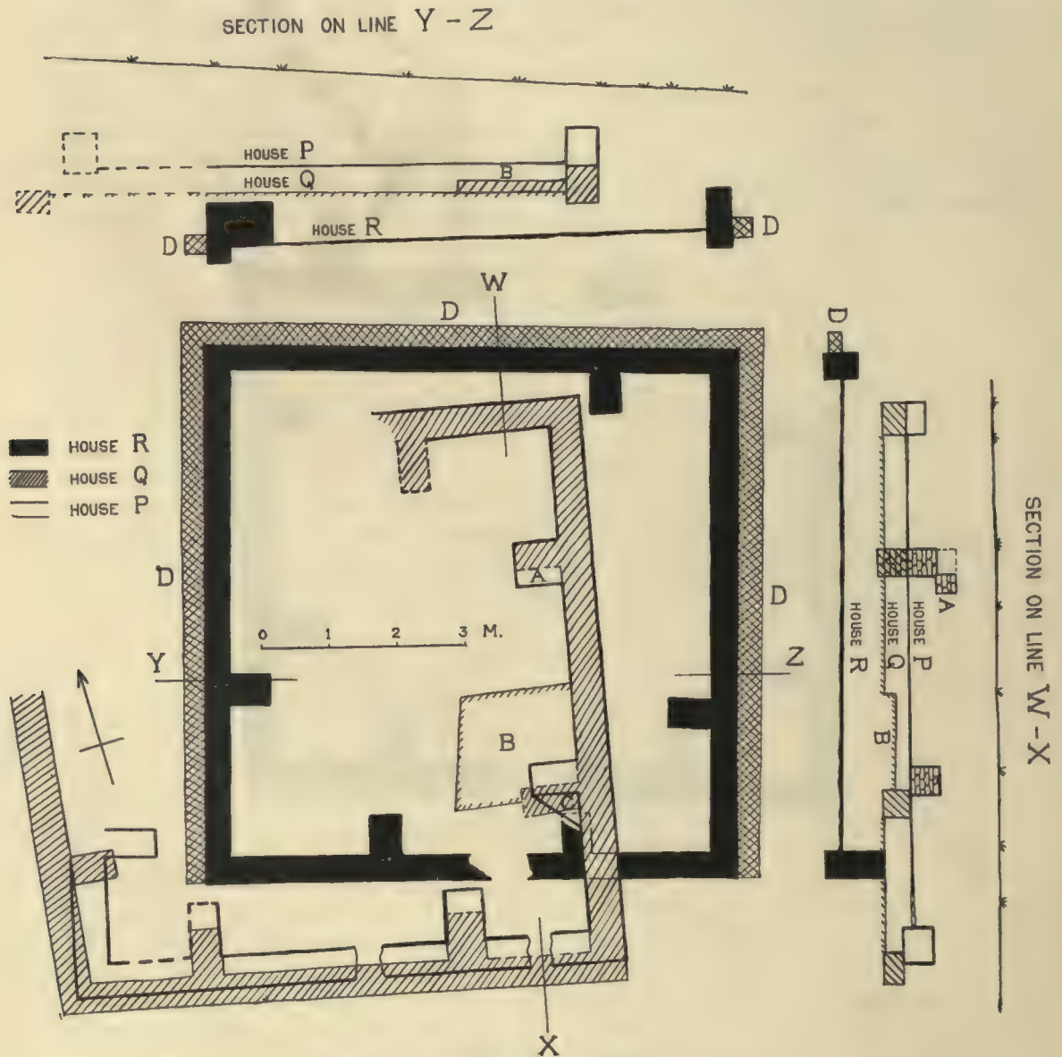
FIG. 65. Tsangli; plan of Houses P , Q , R .
